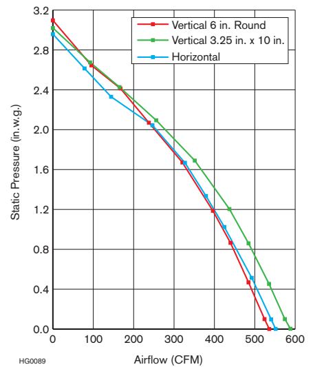
Airflow Performance at High Speed
