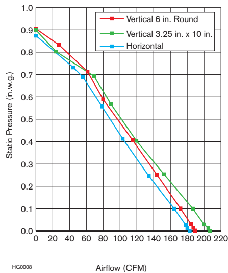
Airflow Performance at Working Speed
